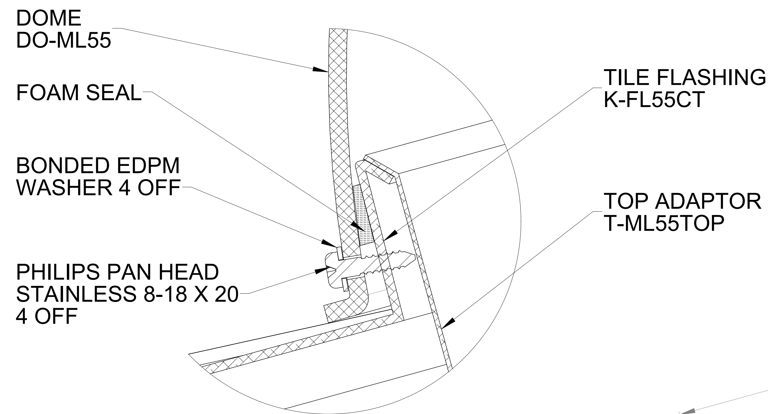
DETAIL B SCALE 2 : 1
