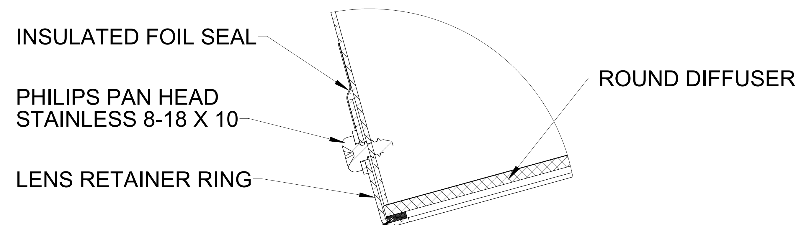
DETAIL C SCALE 2 : 1
