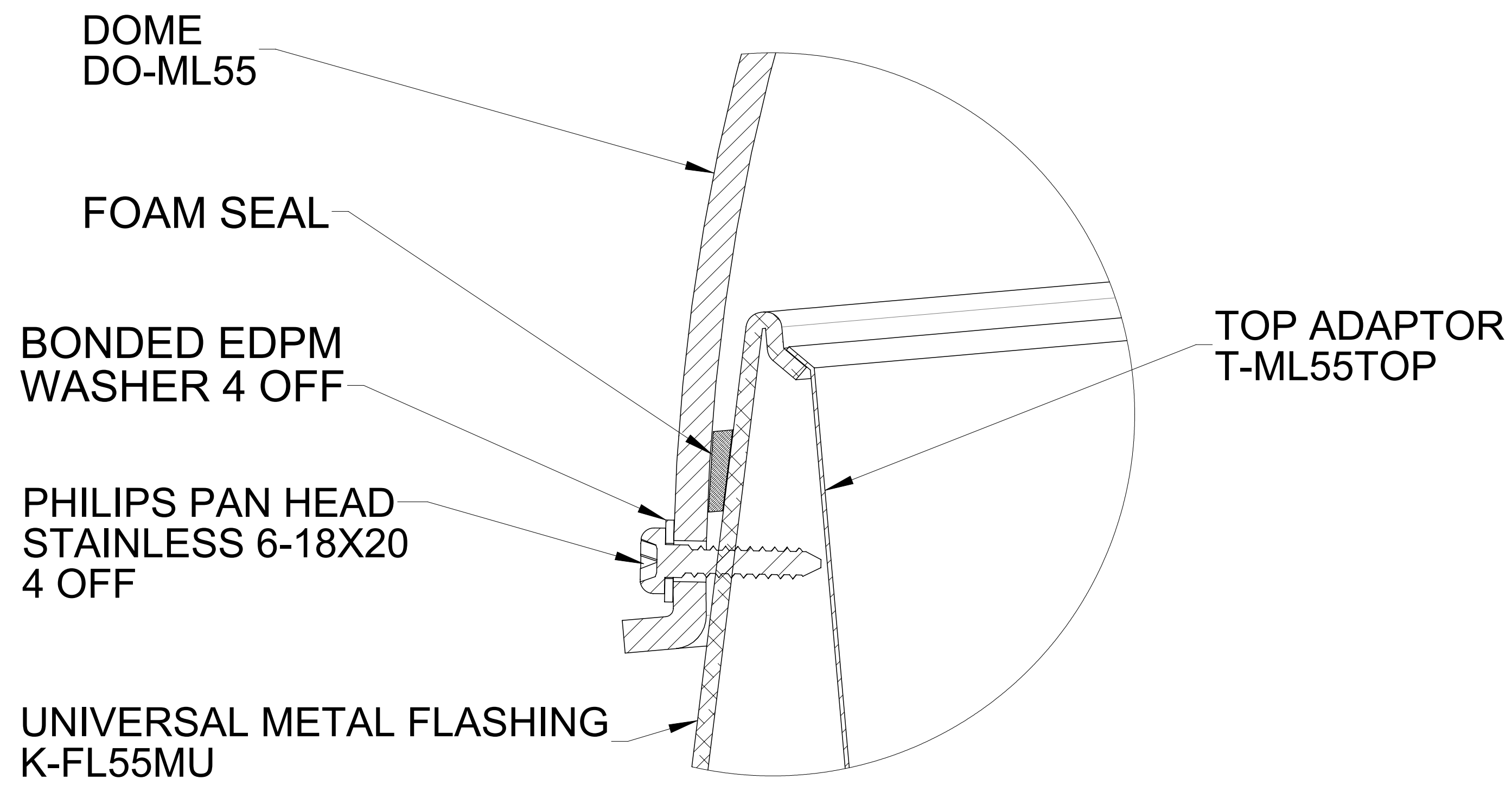
DETAIL B SCALE 2 : 1
